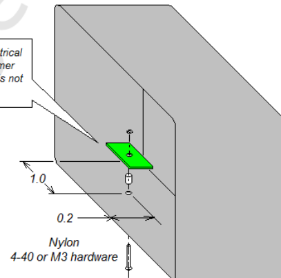
Dimmer control board mounting.
