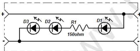
Typical Monochrome LED Segment
